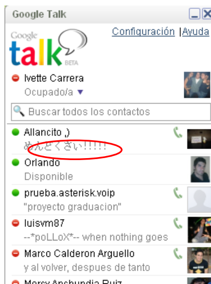
Figura 4.17: Cliente Gtalk
