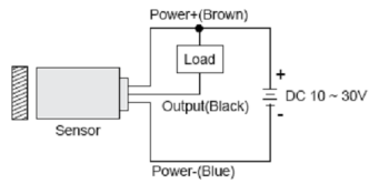
< NPN OUTPUT >
