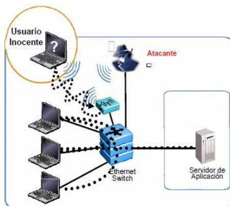
Figura 3.7 ARP Spoofing
