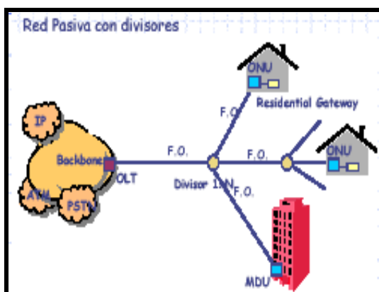
FIGURA 1.17: Red PON
