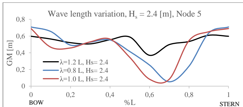
Fig. 3. GMt for different positions of the crest along the vessel. H_s = 2.4 [m]
