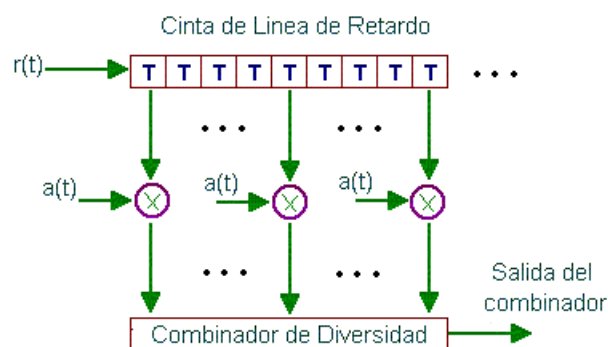
Receptor RAKE
