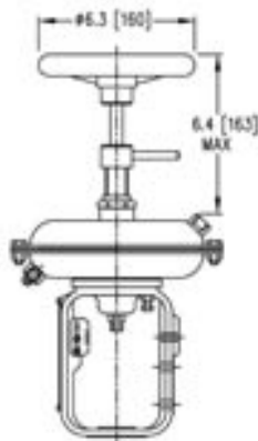
24000C/D FLANGED ATO/Fail Closed Action with Handwheel
