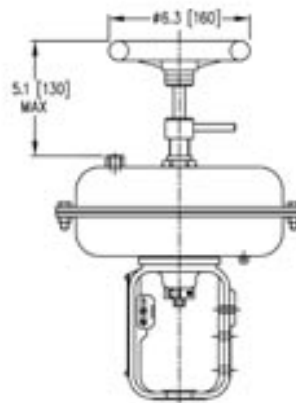
Type 54 ATC/Fail Open Action with Handwheel
