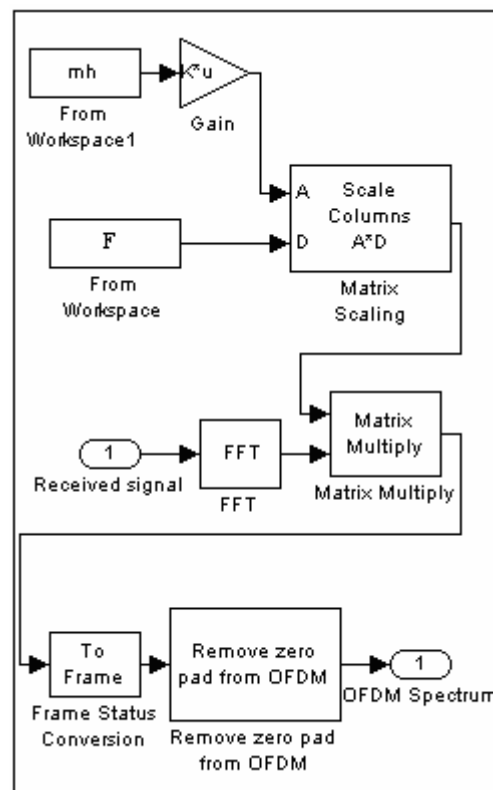
Figura 8. Receptor SOFDM
