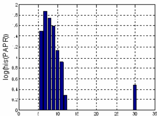
Figura 13. PAPR sin usar spreading
