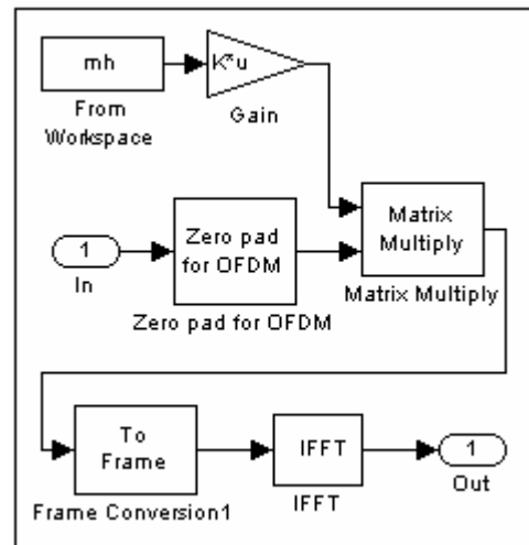
Figura 7. Transmisor SOFDM
