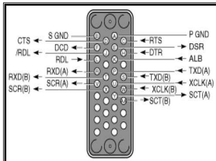
Figura 1.8 Conector Winchester.
