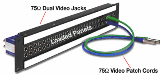
Fig. 4.110. Patch Pannel SDI
