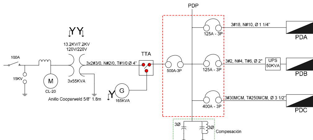
Fig. 6.10 Diagrama Unifilar
