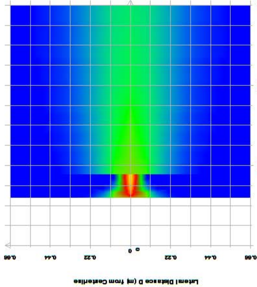
Concentration Profile - Trajectory (s) vs. Lateral Distance D (m) from Plume Centerline
