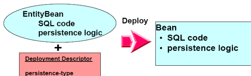
Figura 12. Bean-Managed Persistence
