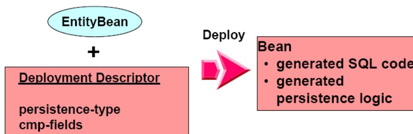
Figura 13. Container-Manged Persistentente
