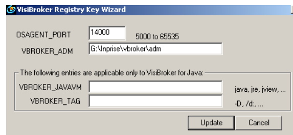
Figura 37: Visibroker Wizard
