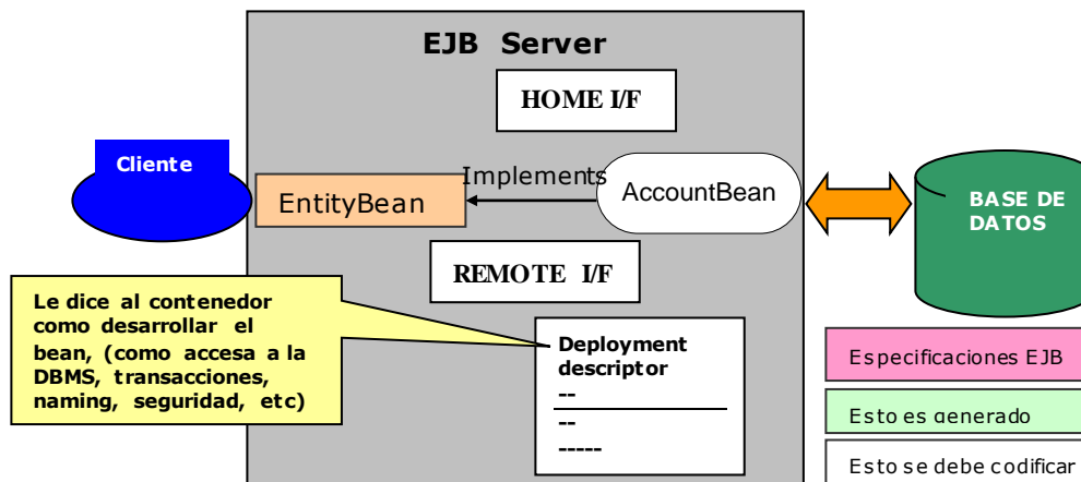
Figura 16. Deployment Descriptor
