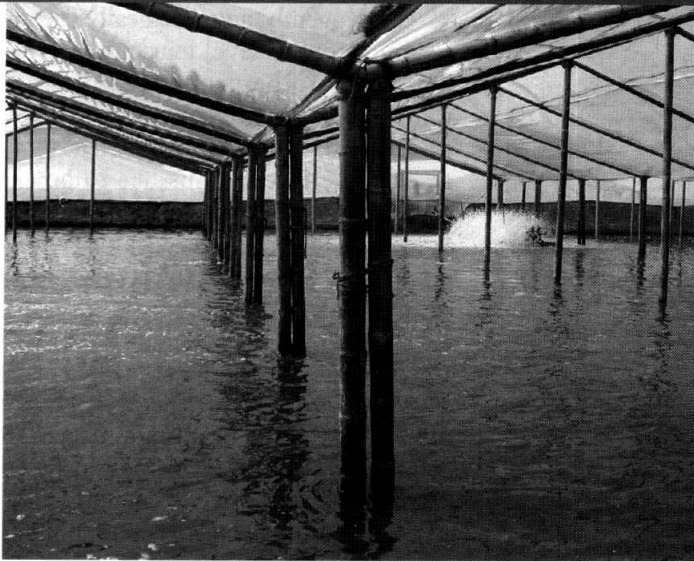
Pond covers built with bamboo poles (left) are functional and initially inexpensive, but may not last as long as covers constructed with more permanent materials.
