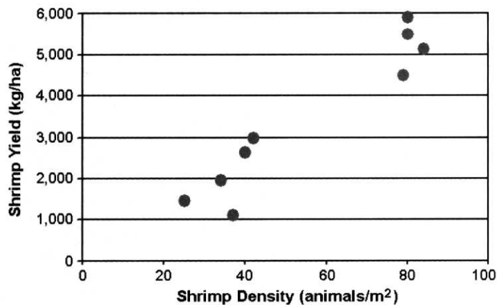
Figure 2. Relationship of shrimp yield and stocking density in greenhouse shrimp growout production trials.
