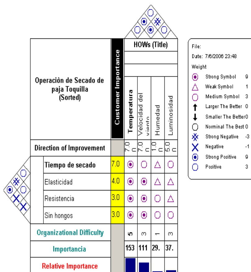
Figura 4.3 QFD
