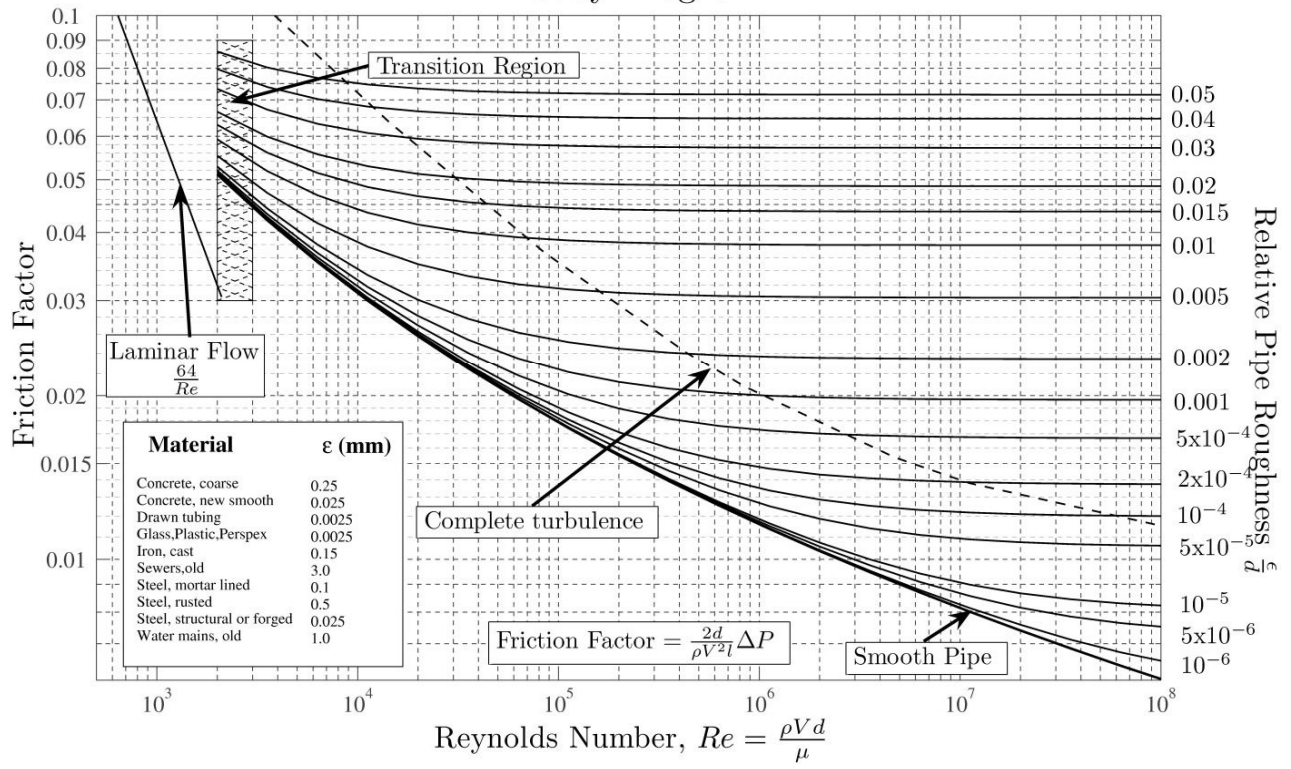
Moody Diagram
