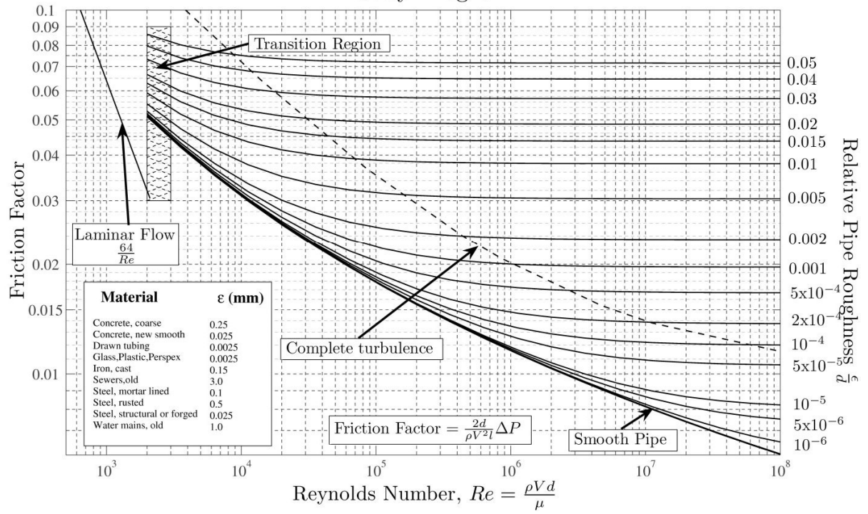
Moody Diagram
