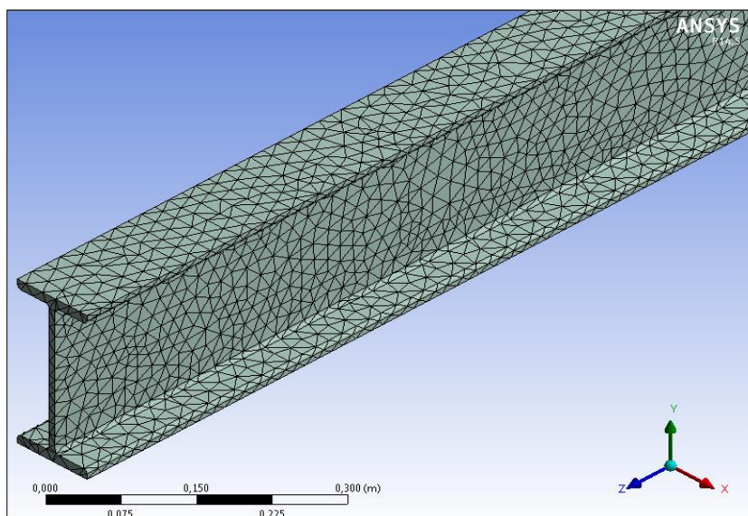
FIGURA 3.20. MALLADO TETRAÉDRICO PATCH INDEPENDENT
