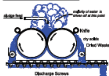
Cross-Section of Double Drum Dryer
