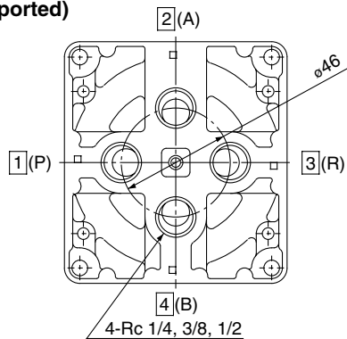
VH43□-02 to 04 (Bottom ported)
