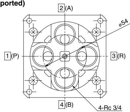
VH43□-06 (Bottom ported)
