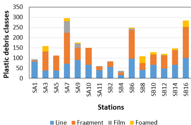
Figure 4: Identity and class of plastic debris collected in each station.
