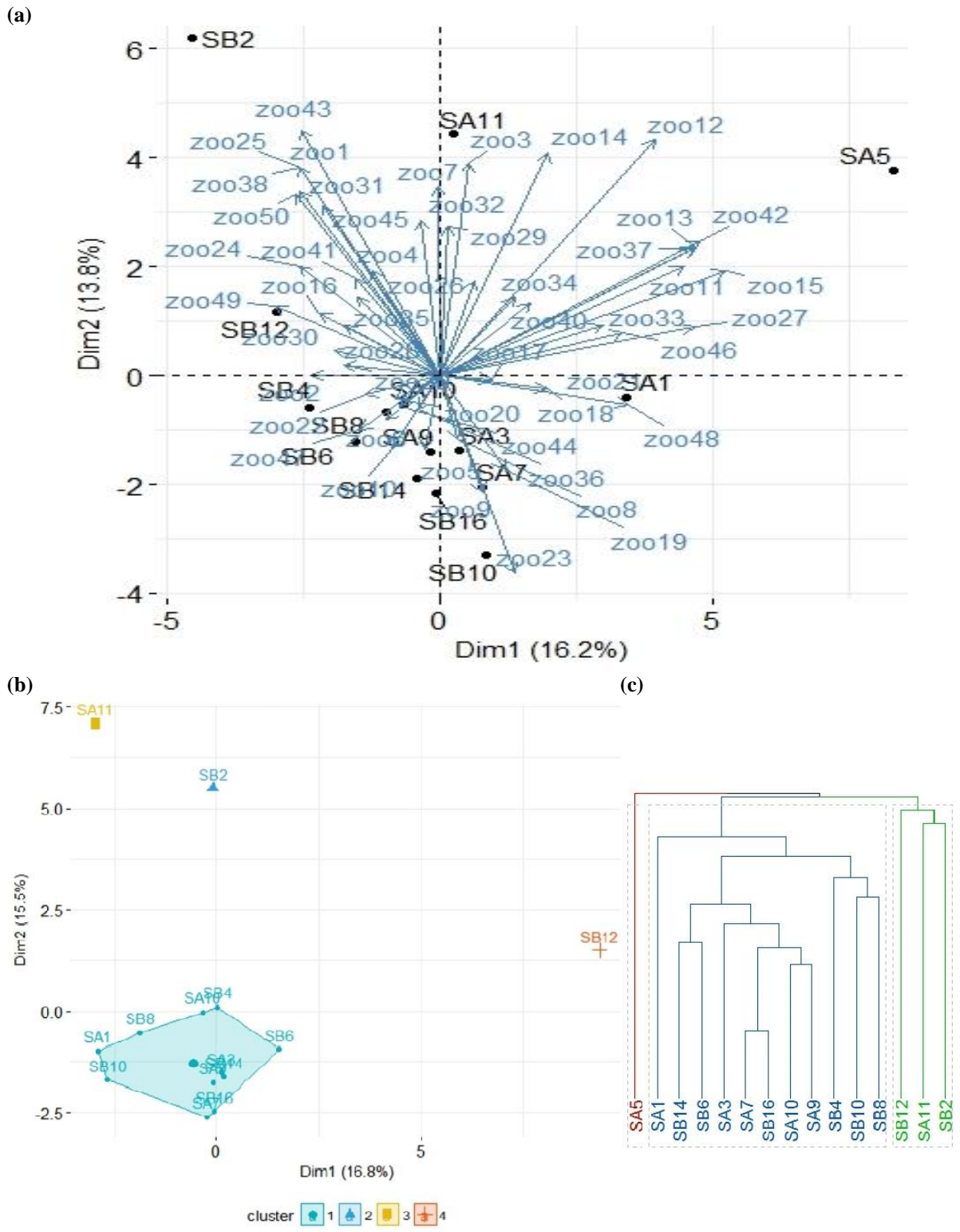
Figure 3 Exposure to including zooplankton species for each station: (a) PCA analysis, all fifty zooplankton species are represented in this bi-plot by a vector and statios by points. First principal component(Dim1) is represented by horizontal axis, while second principal component (Dim2) is represented by vertical axes. (b) Cluster analysis, represent the most related stations. (c) Dendrogram showing the similarities and differences within station, shorter liner are stations very closely related.
