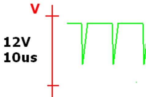
Figura 4.5.4 TP448 Oscilograma
