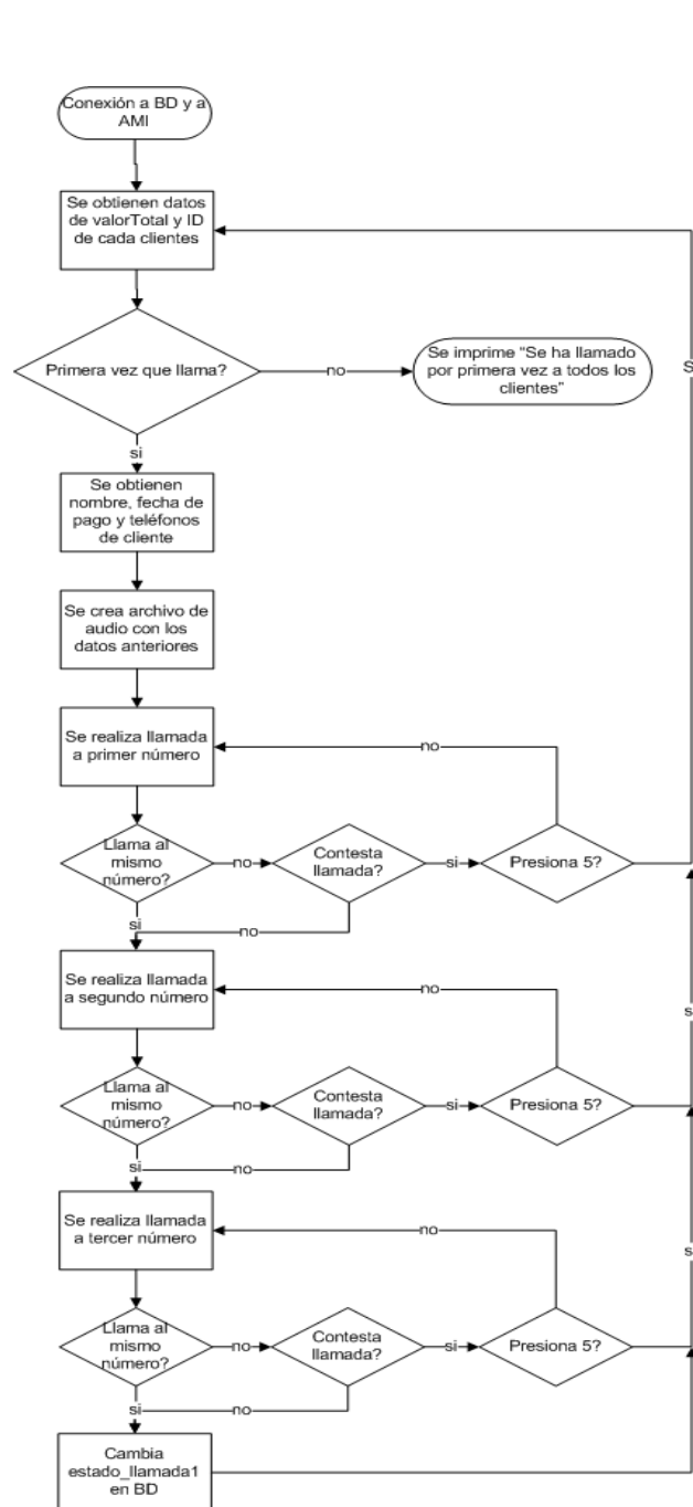
Fig 3.4 Diagrama de flujo de scripts amiCanal#.php, ami2Canal#.php
