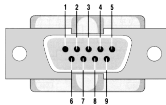
Figura 2.5 - CONECTOR DB9
