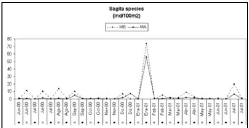
Figura 50: Sagitta species
