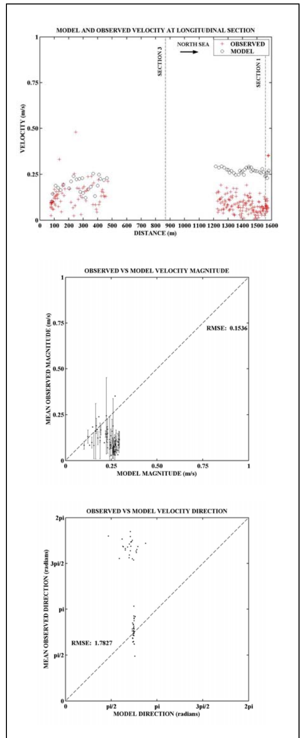
Figure D-6: Model and Observed velocity at 20:00
