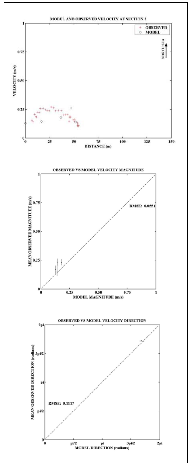
Figure D-26: Model and Observed velocity at 19:30 at Section 3
