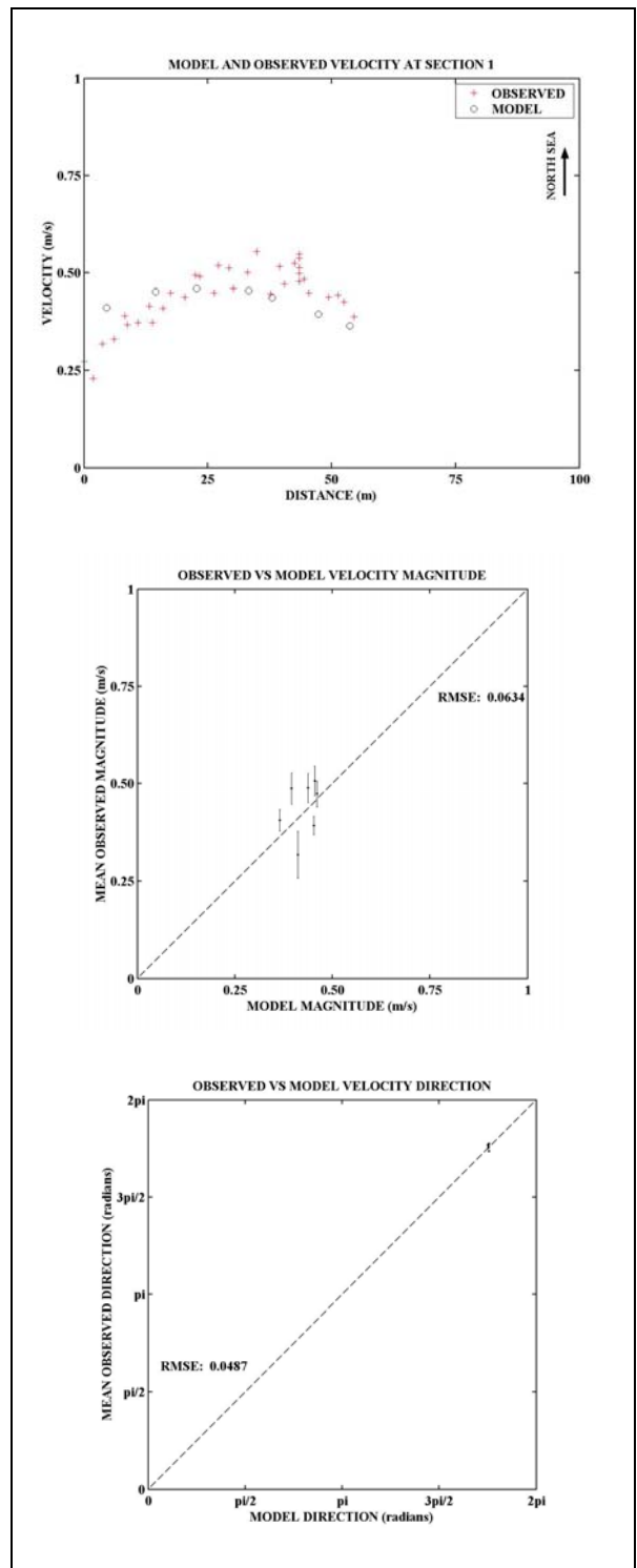
Figure D-13: Model and Observed velocity at 19:00 at Section 1
