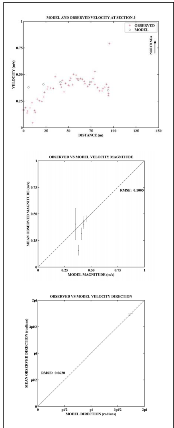
Figure D-24: Model and Observed velocity at 16:30 at Section 3
