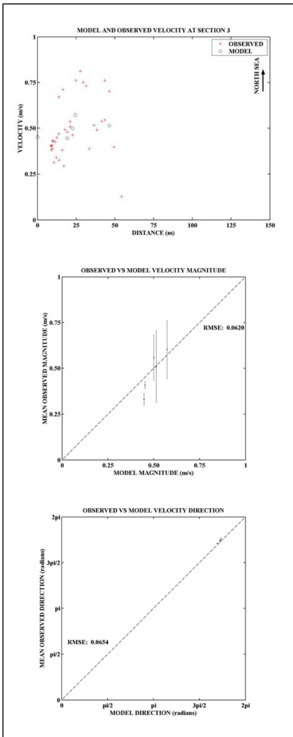
Figure D-25: Model and Observed velocity at 18:00 at Section 3
