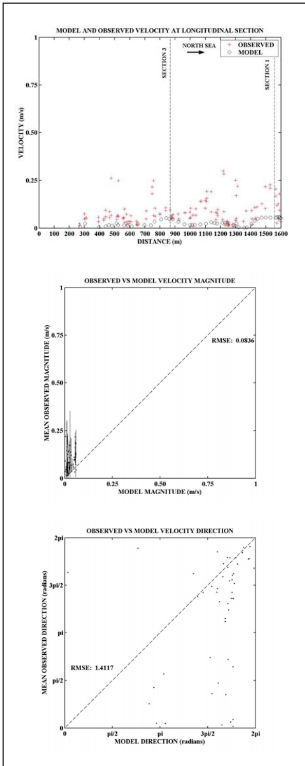
Figure D-1: Model and Observed velocity at 13:30
