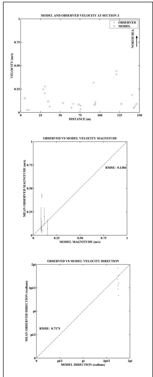
Figure D-22: Model and Observed velocity at 14:00 at Section 3
