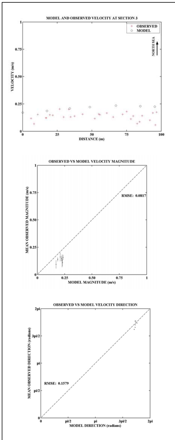
Figure D-23: Model and Observed velocity at 15:00 at Section 3
