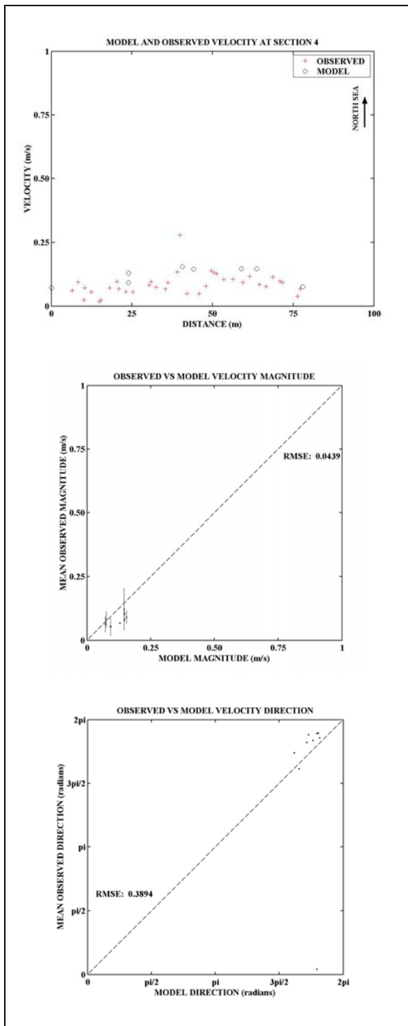
Figure D-30: Model and Observed velocity at 17:00 at Section 4
