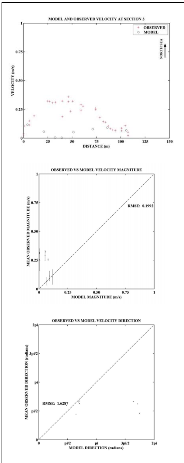
Figure D-21: Model and Observed velocity at 12:30 at Section 3
