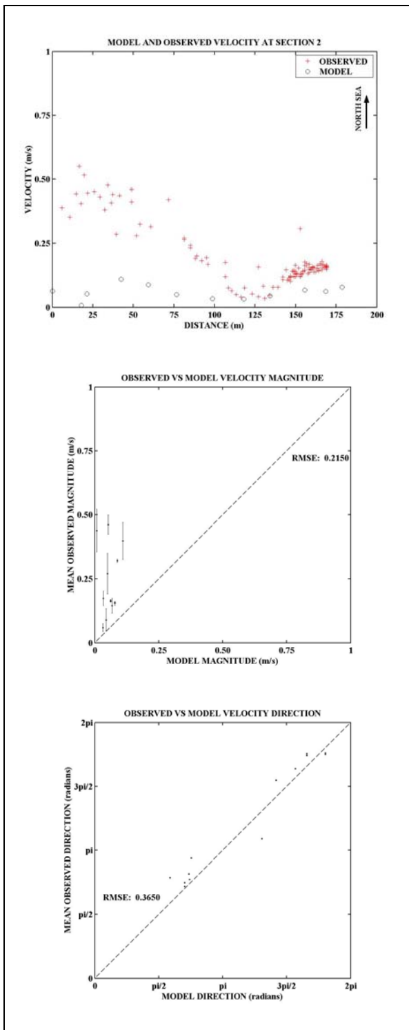
Figure D-15: Model and Observed velocity at 12:30 at Section 2
