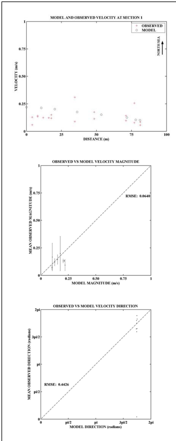
Figure D-10: Model and Observed velocity at 14:00 at Section 1
