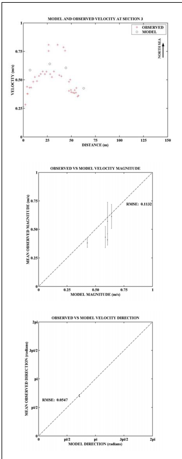
Figure D-27: Model and Observed velocity at 21:00 at Section 3
