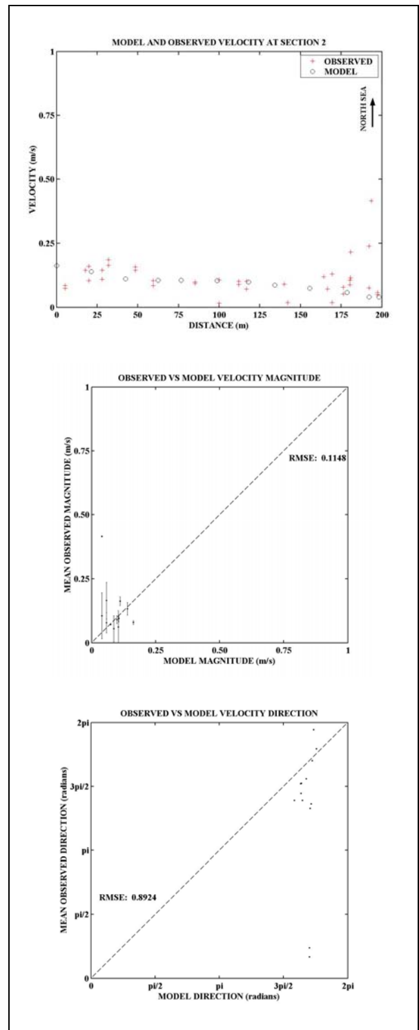
Figure D-16: Model and Observed velocity at 14:00 at Section 2
