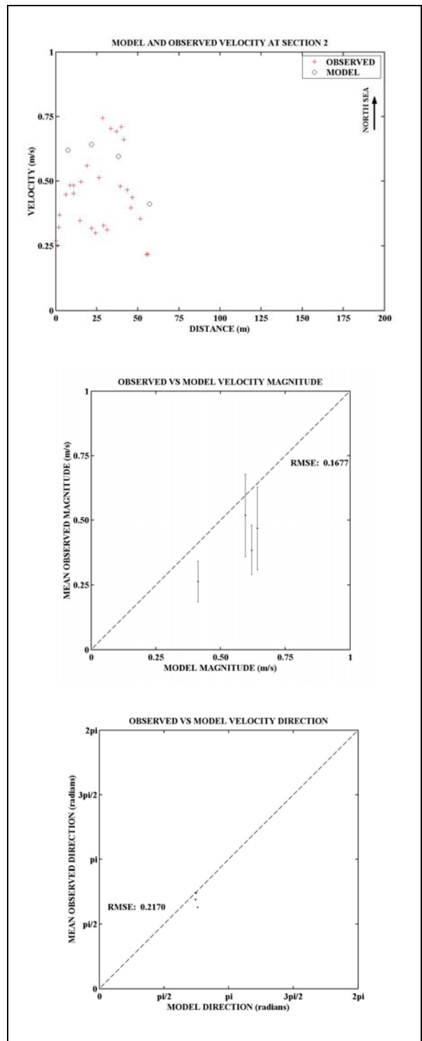
Figure D-20: Model and Observed velocity at 21:00 at Section 2
