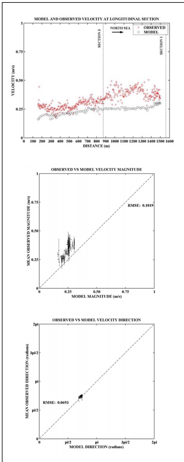
Figure D-9: Model and Observed velocity at 21:30
