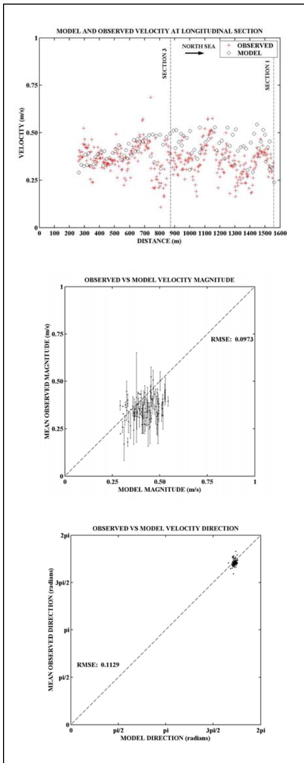
Figure D-3: Model and Observed velocity at 17:30
