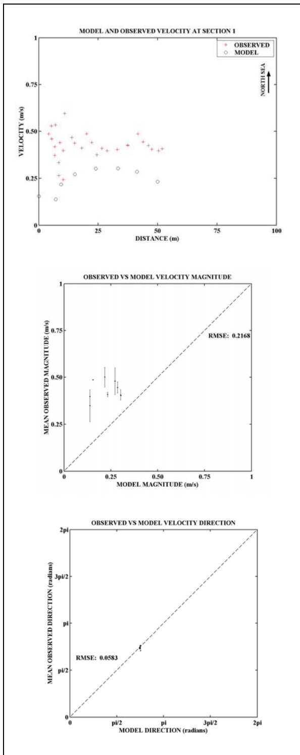
Figure D-14: Model and Observed velocity at 21:30 at Section 1
