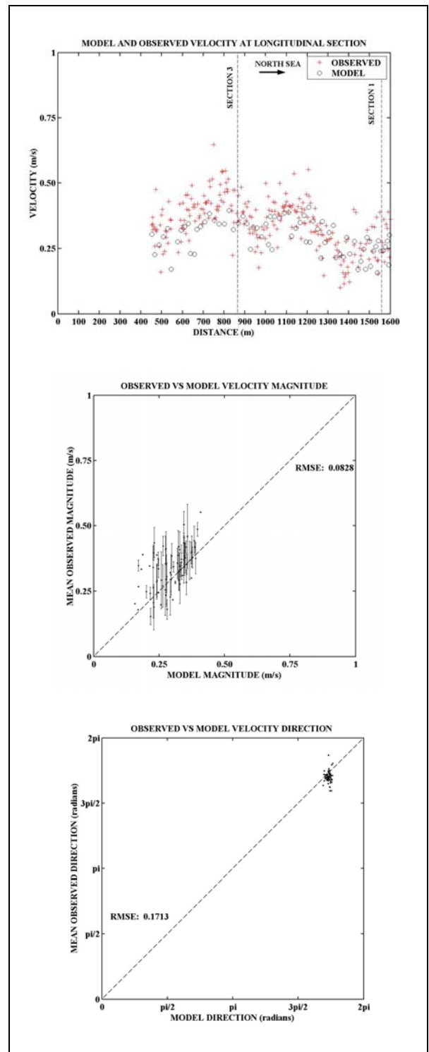
Figure D-4: Model and Observed velocity at 19:00
