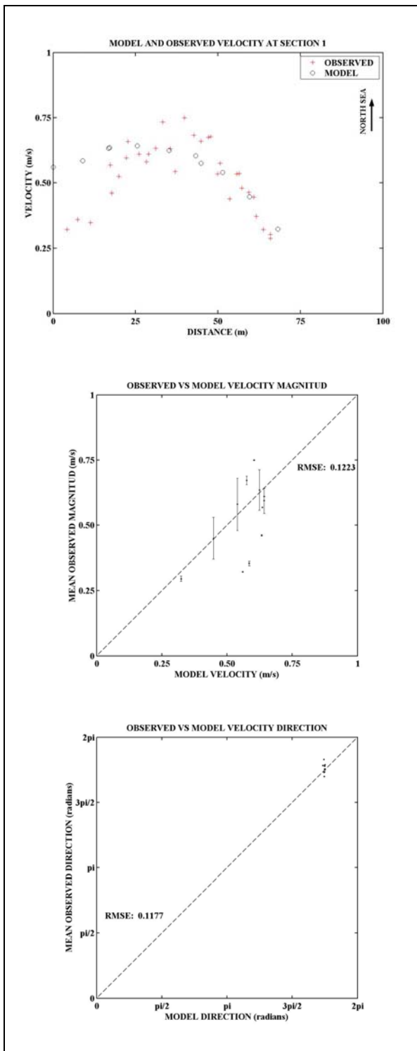
Figure D-12: Model and Observed velocity at 17:30 at Section 1
