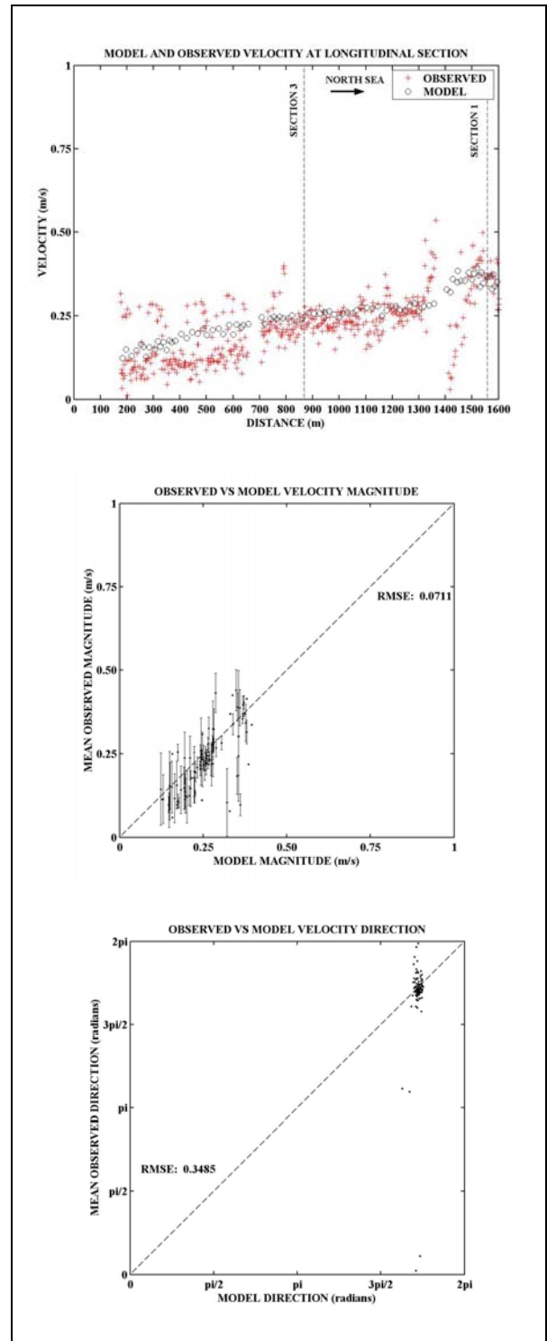
Figure D-2: Model and Observed velocity at 15:00
