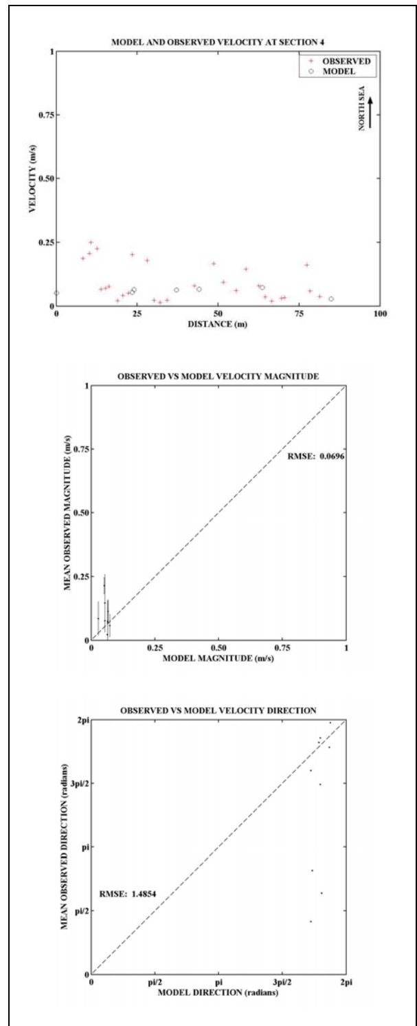
Figure D-29: Model and Observed velocity at 14:30 at Section 4
