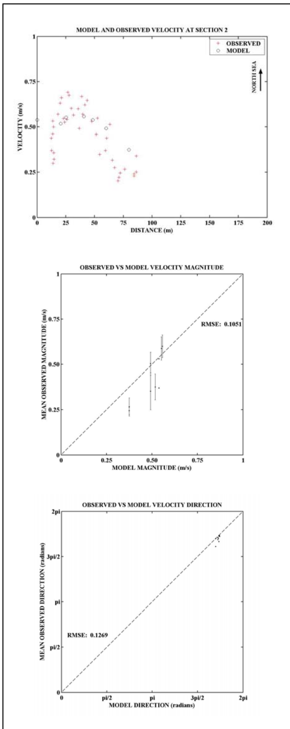
Figure D-17: Model and Observed velocity at 16:00 at Section 2
