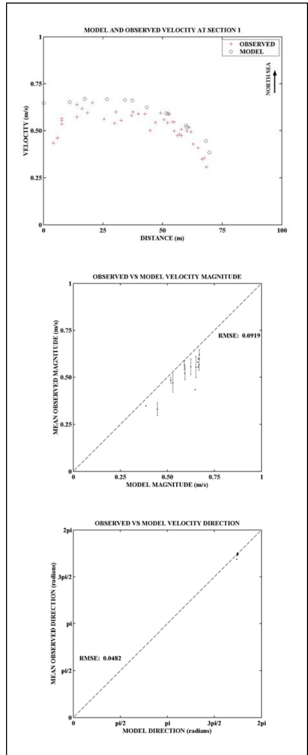
Figure D-11: Model and Observed velocity at 16:00 at Section 1
