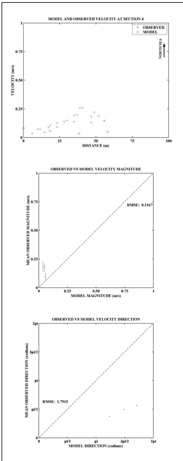
Figure D-28: Model and Observed velocity at 12:30 at Section 4
