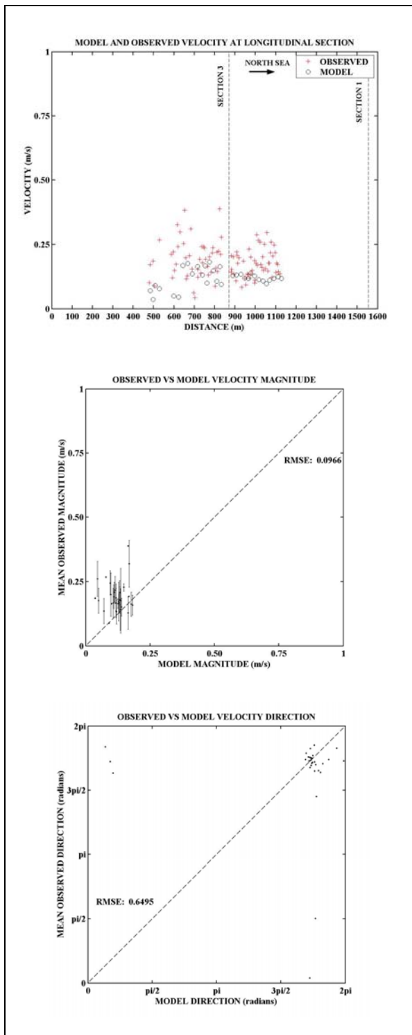
Figure D-5: Model and Observed velocity at 19:30
