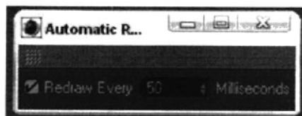
Figura 6-51: Automatic Redraw.
