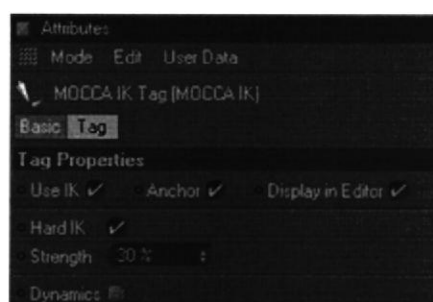
Figura 6-46: Anchor.
