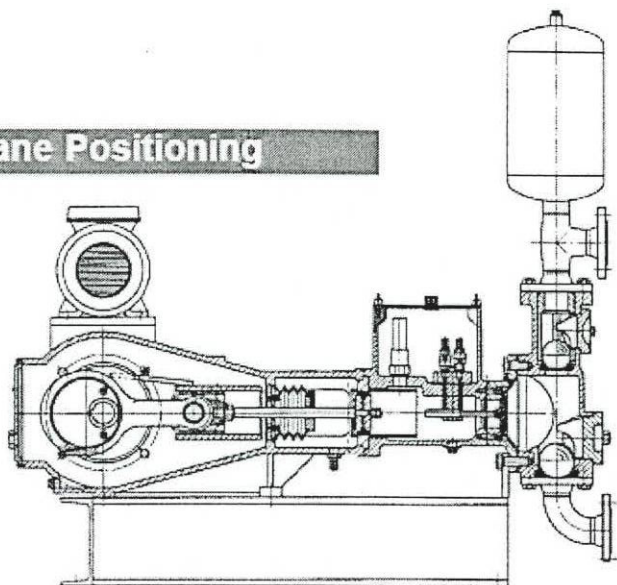
Single-acting design
