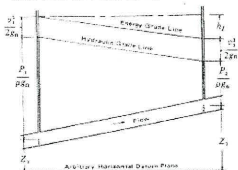
Figure 1-4 Energy Balance for Two Points in a Fluid
