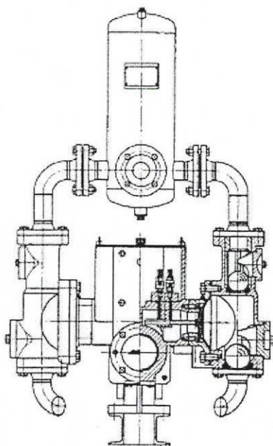
Double-acting design
