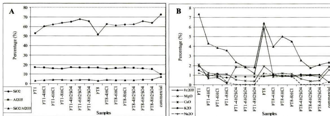
Figure 5.3- Chemical composition of commercial, natural, and acid activation samples. A: % SiO 2 , % Al 2 O 3 and SiO 2 /Al 2 O 3 ratio; B: % Fe 2 O 3 , %MgO, %CaO, %K 2 O, %Na 2 O.
