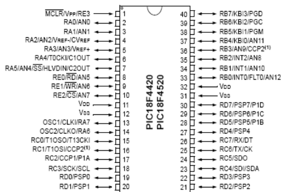
Figura 5. PIC18F4550.
