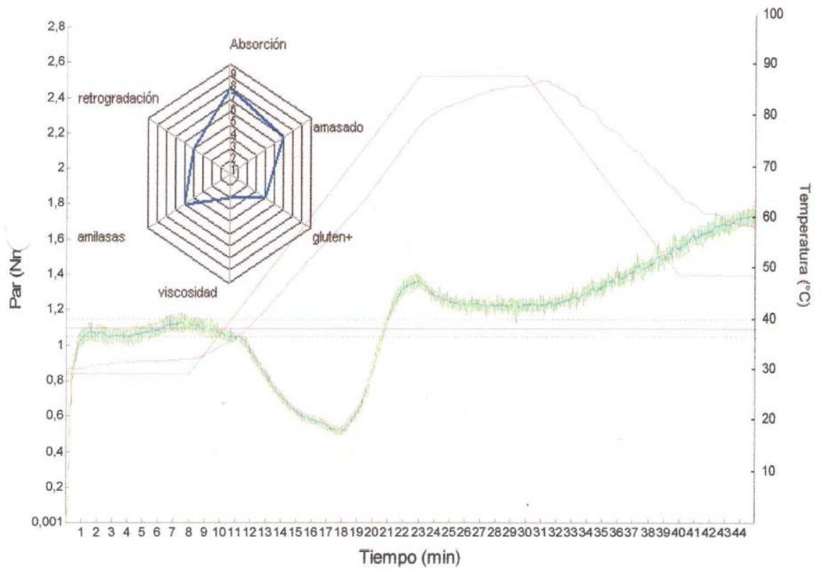
Figura 2.9 Mixograma Patron
