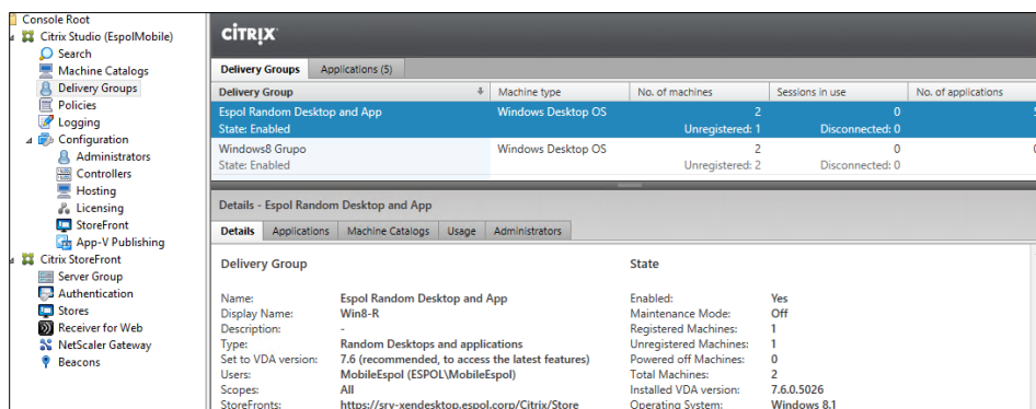
Figura 2.16: Delivery Groups configurados en XenDesktop.
