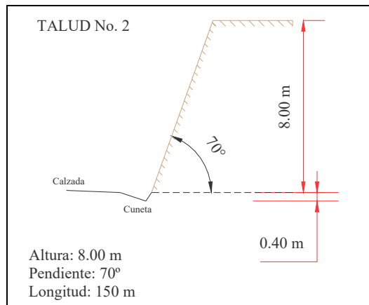
Figura 2.2.2 Talud No. 2
