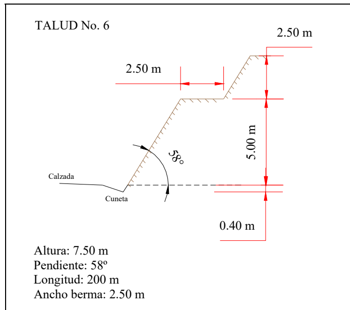
Figura 2.2.6 Talud No. 6
