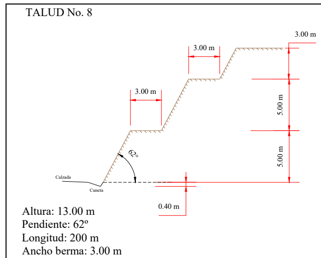
Figura 2.2.8 Talud No. 8
