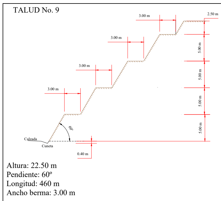
Figura 2.2.9 Talud No. 9
