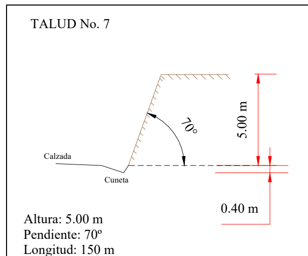
Figura 2.2.7 Talud No. 7
