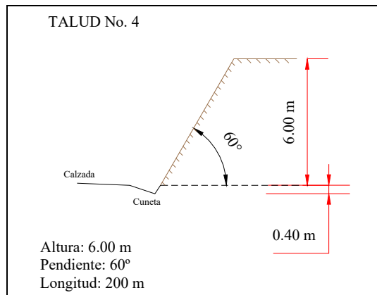
Figura 2.2.4 Talud No. 4
