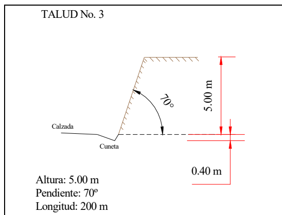
Figura 2.2.3 Talud No. 3
