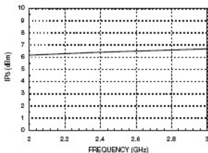
Rx Output Third Order Intercept Point
