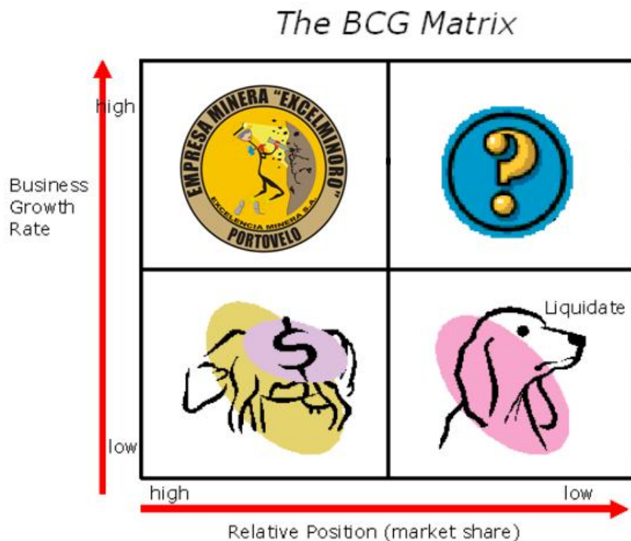
Figura 5: Matrix BCG
