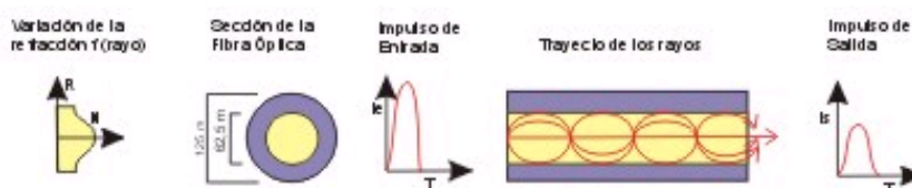
Figura # 4.4 Fibra multimodo gradiente gradual
