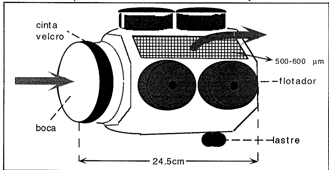
Figura No. 4. Recipiente recolector o Cubilete.
