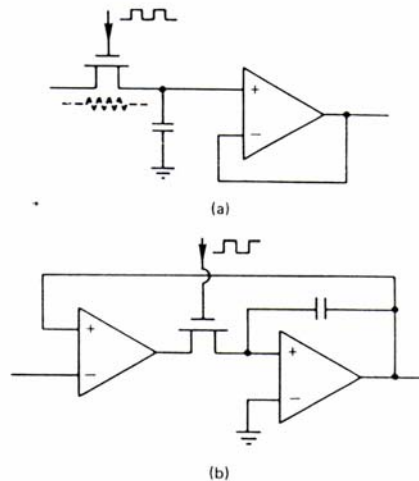
Figura 5.32 Circuitos Sample and Hold
