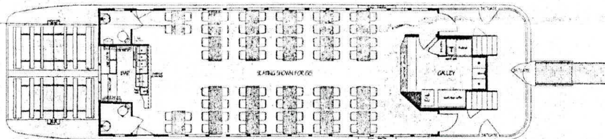
MAIN DECK ARRANGEMENT
